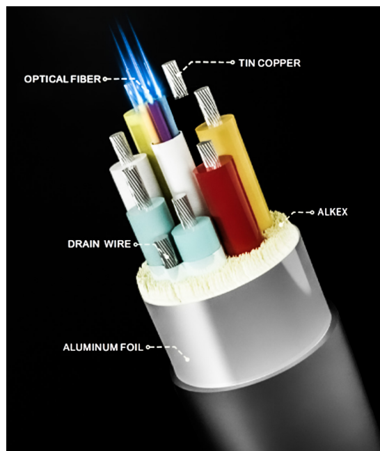
Cable cross-section
